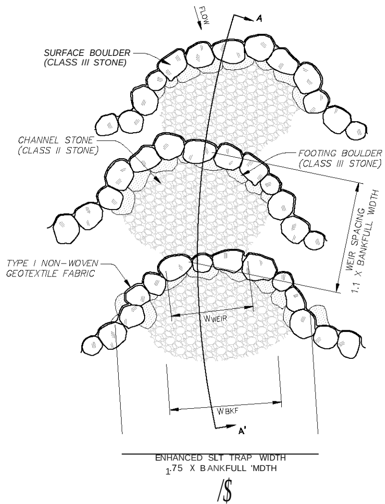
ENHANCED SILT TRAP PLAN
